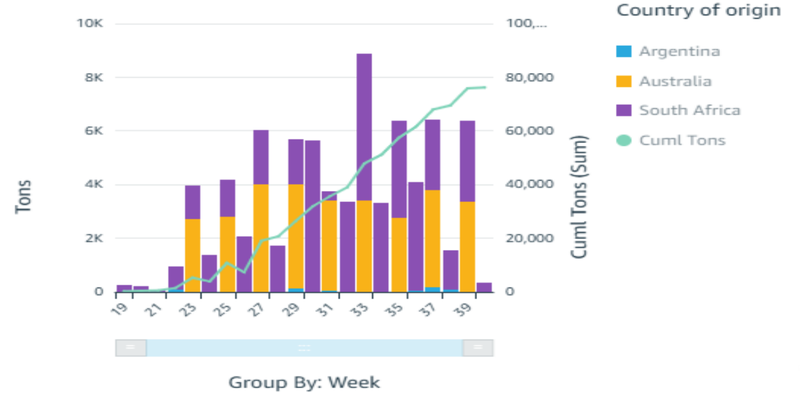
Weekly Citrus tons exported to South East Asia
